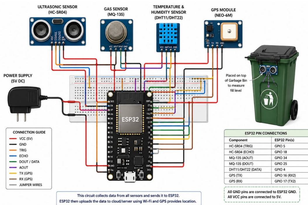
Figure : 2 Image of Circuit Diagram
